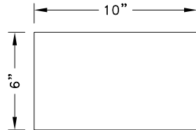
Plate A 12g ASTM A653 SS Grade 33 G60 Bare Metal Thickness: t = 0.0966"
